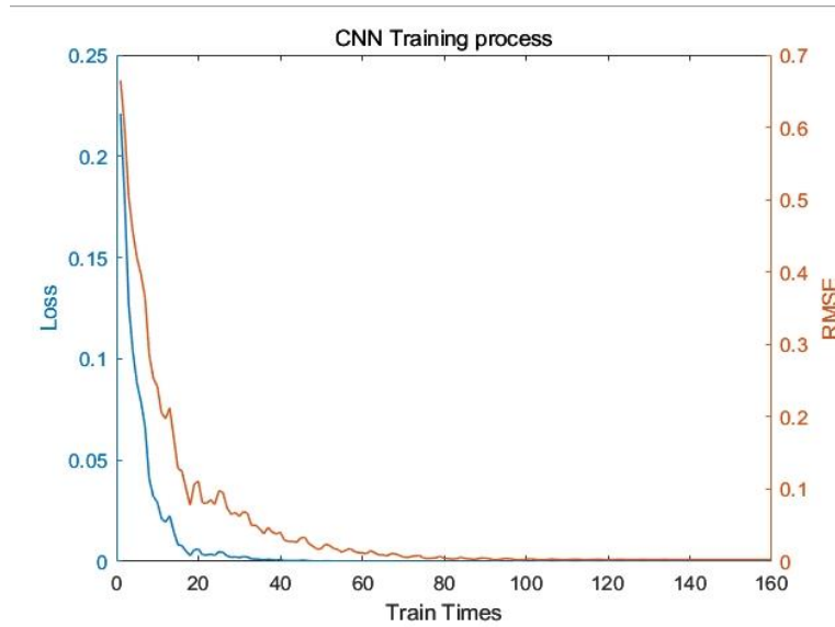
Figure 7. The training process of CNN.
