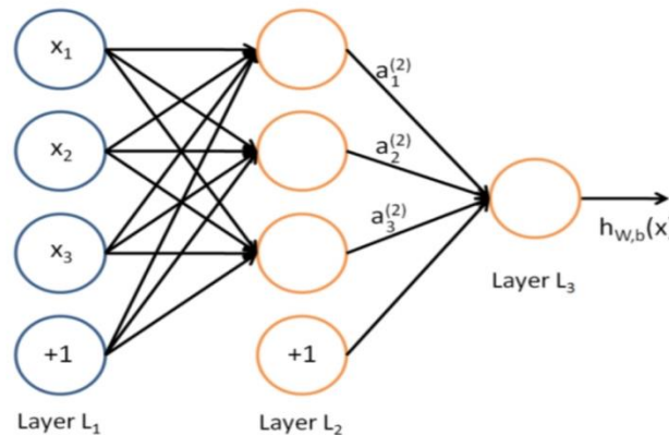
Figure 3. Mathematical structure and bionic mechanism of feedforward neural network model.
