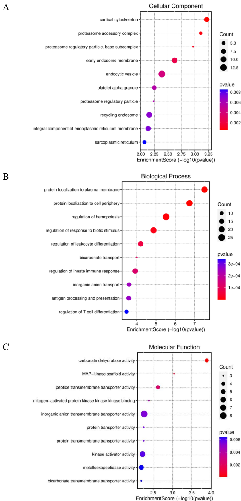
Fig. 2 The result of GO analysis for the different expressed genes by microglia in AD.
