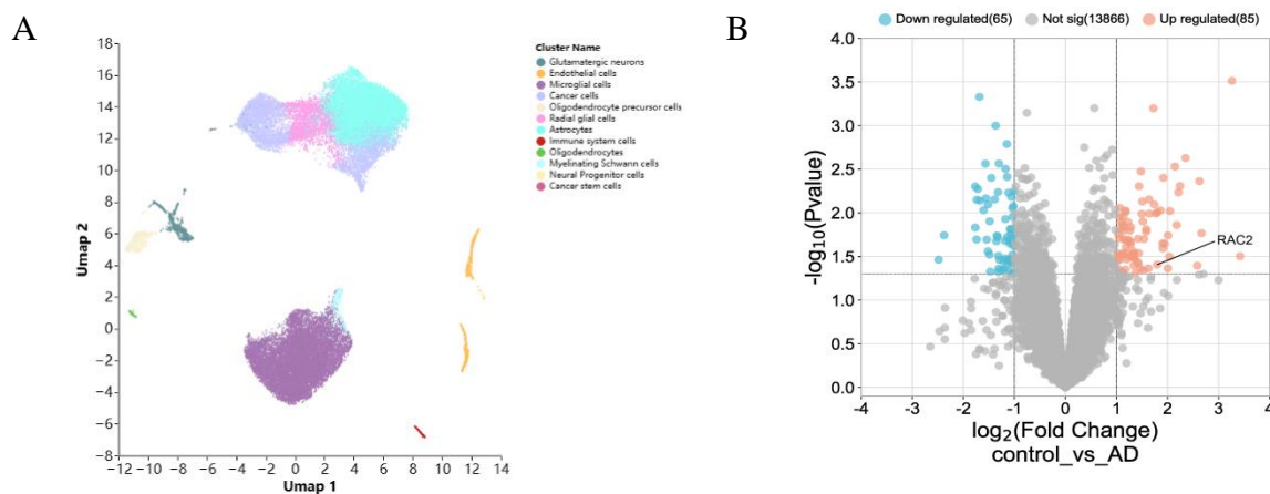
Fig. 1 Single-cell RNA sequencing of the cortex in AD patients and control brains revealed changes in gene expression.
