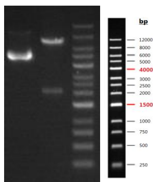
Fig. 3 DNA gel electrophoresis indicated that RAC2 overexpression plasmid was successfully constructed
