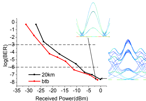
Fig. 3 The BER v/s received power curves of CRZ-4PAM signals after 20km SMF transmission
