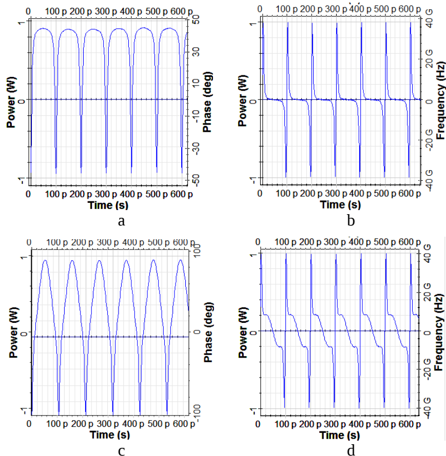
Fig. 2 The time-domain phase change diagram(a) and time-domain chirp change diagram(b) of RZ - 4PAM signals, The time-domain phase change diagram(c) and time-domain chirp change diagram(d) of CRZ -4PAM signals.
