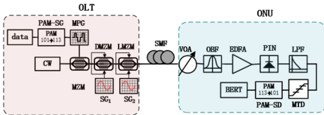
Fig. 1 System setup for the CRZ-4PAM downlink transmission (CW: Continuous wave; PAM-SG:PAM sequence generator; MPG:M-ary pulse generator; DMZM: dual-arm Mach-Zehnder modulator; LMZM: LiNbO 3 Mach-Zehnder modulator; SG: sine generator; SMF:single mode fiber; VOA: variable optical attenuator; OBF:Bessel Optical filter; EDFA:erbium-doped optical fiber amplifier; PIN:Photo detector; MZM: Mach-Zehnder Modulator; LPF: low pass filter; MTD: M-ary threshold detector; PAM-SD: PAM sequence decoder; BERT: bit error rate tester.)
