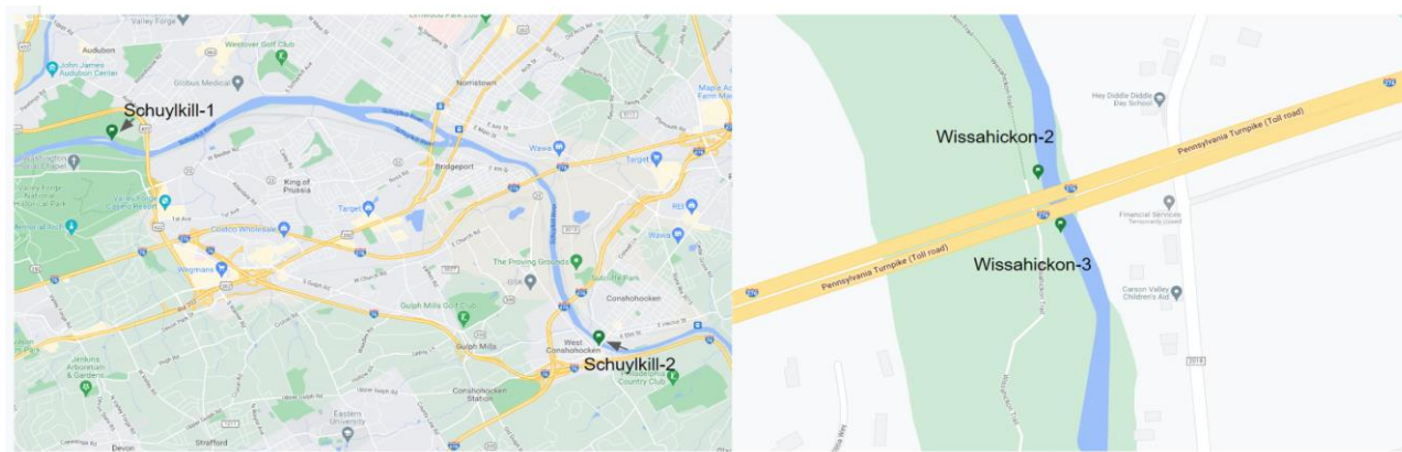
Fig. 2 The locations of samples graphed on Google Maps.
