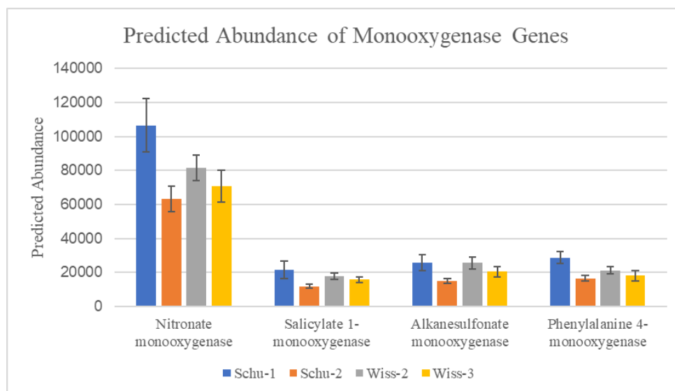
Fig. 11 The predicted abundance of several monooxygenase genes in four locations. Error bars indicate standard deviation.
