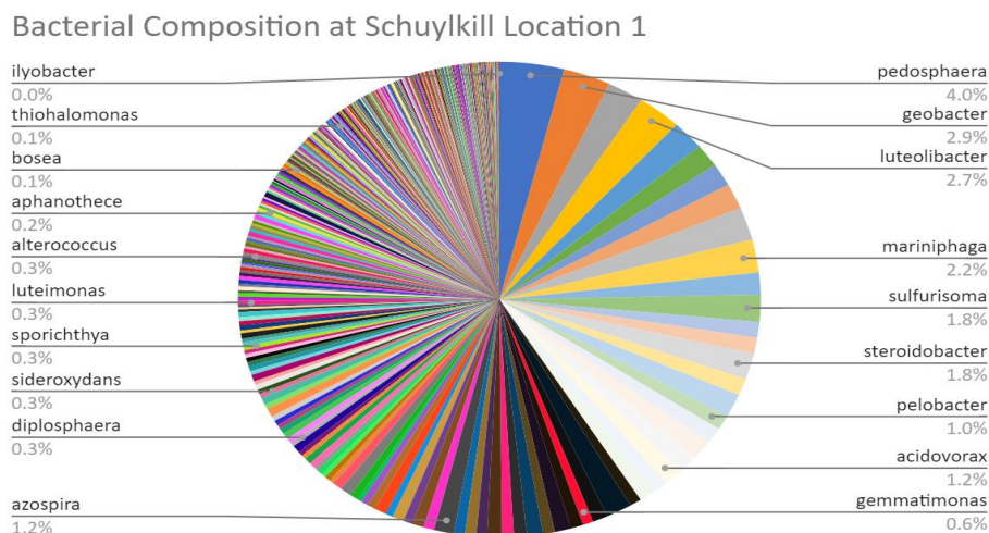
Fig. 3 The bacterial composition at Schuylkill location 1, with specific taxonomic abundance displayed for each prominent genus of bacteria.
