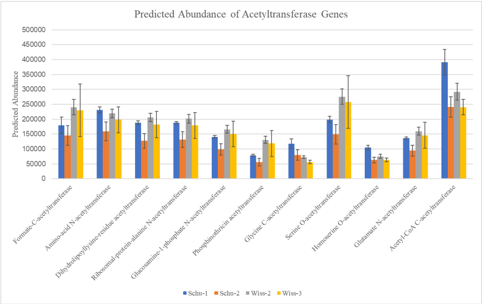
Fig. 8 The predicted abundance of several acetyltransferase genes in four locations. Error bars indicate standard deviation.
