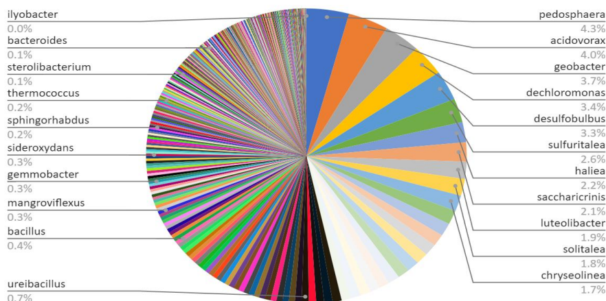
Fig. 4 The bacterial composition at Schuylkill location 2, with specific taxonomic abundance displayed for each prominent genus of bacteria.
