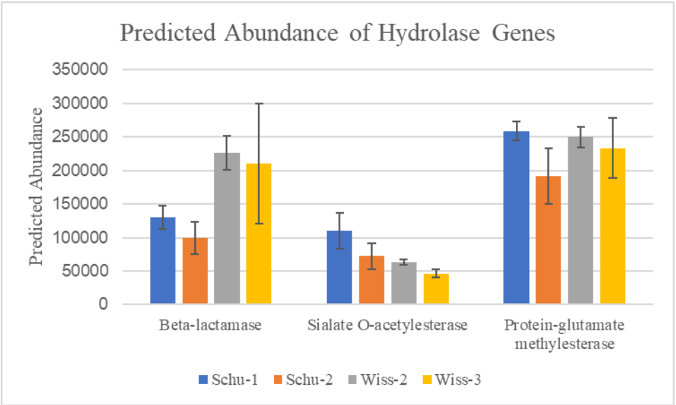
Fig. 7 The predicted abundance of several hydrolase genes in four locations. Error bars indicate standard deviation.
