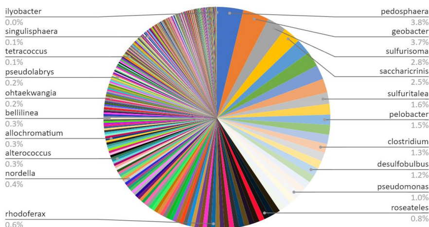
Bacterial Composition at Wissahickon Location 2
