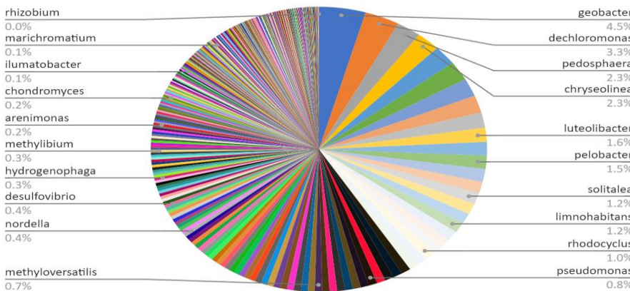
Fig. 6 The bacterial composition at Wissahickon location 3, with specific taxonomic abundance displayed for each prominent genus of bacteria.
