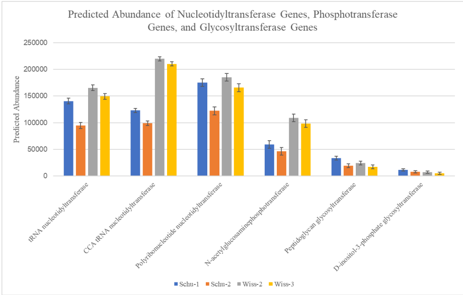
Fig. 9 The predicted abundance of several nucleotidyltransferase genes, phosphotransferase genes, and glycosyltransferase genes in four locations. Error bars indicate standard deviation.
