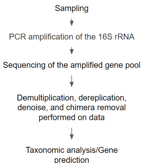
Fig. 1 The main processes of 16s rRNA sequencing that was employed in this study.
