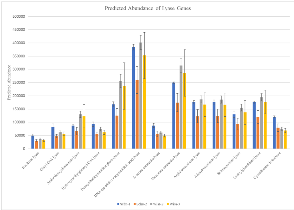
Fig. 10 The predicted abundance of several lyase genes in four locations. Error bars indicate standard deviation.
