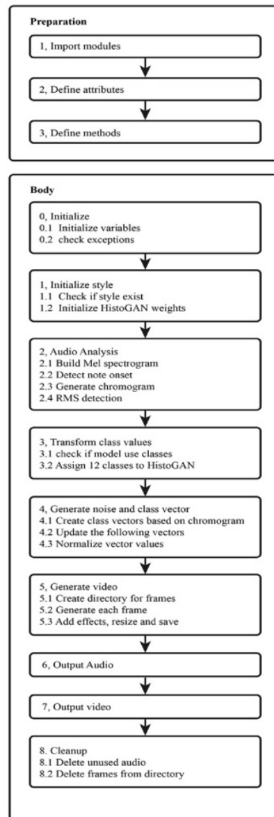
Fig 5. The AI Color Organ algorithm.
