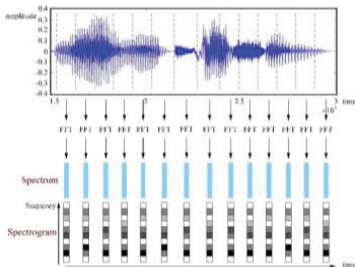
Figure 3. The 2D spectrogram
