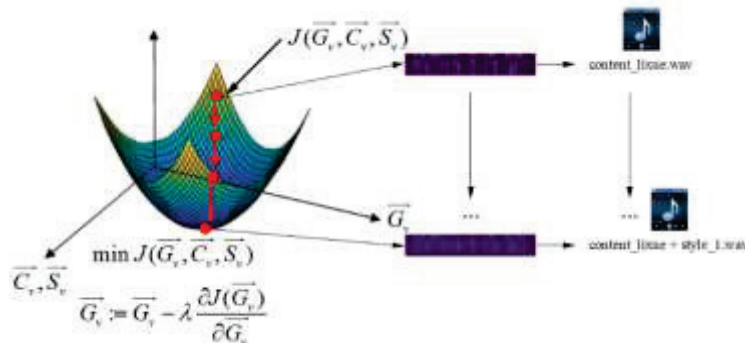
Figure 8. The iteration acquisition diagram for the audio file of generated speech
