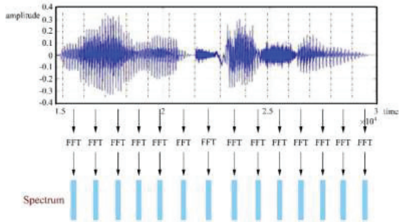
Figure 1. The speech frames
