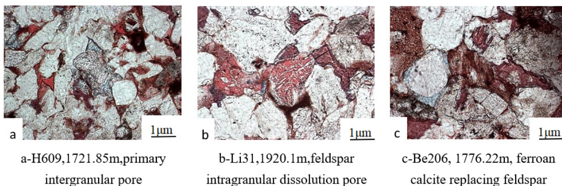
Fig 5. Common pore types in Chang 3 reservoir in Baibao area
