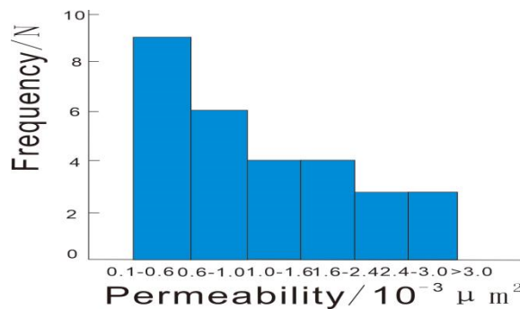
Fig 3. Histogram of Reservoir Permeability Distribution
