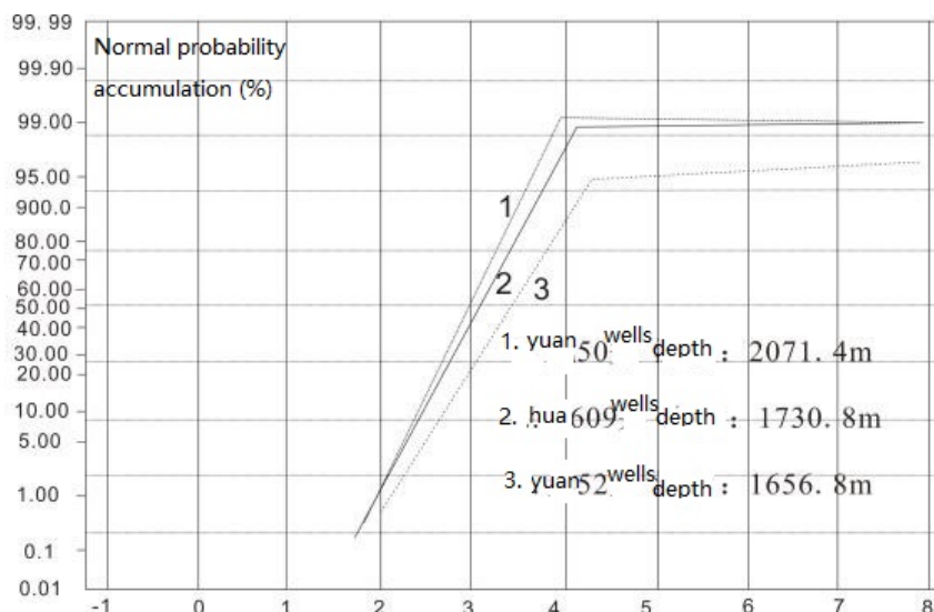
Fig 6. Cumulative probability curve of grain size for Chang 3 sandstone in the Baibao area
