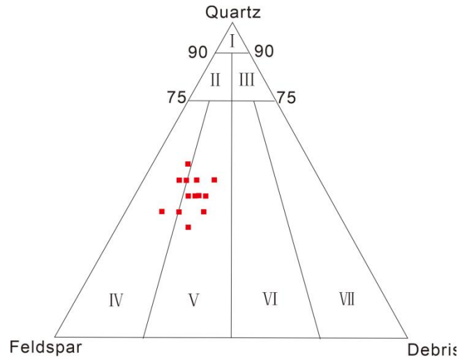
Fig 1. Triangle diagram of rock types in the Chang-3 oil reservoir group in the Baibao area
