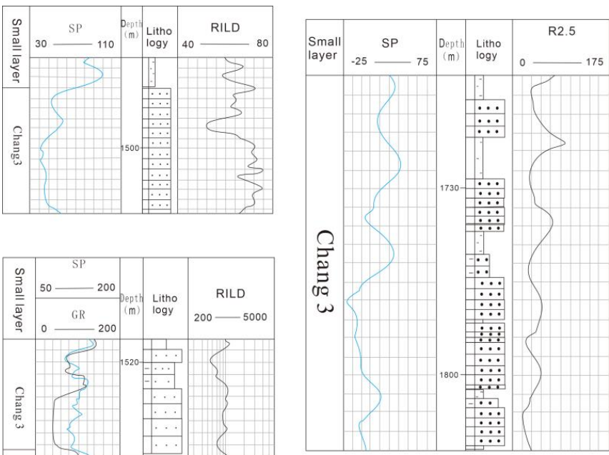
Fig 8. Sedimentary rock electrical characteristics of underwater distributary channels in the delta front
