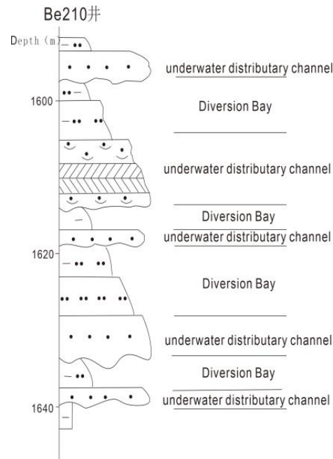
Fig 7. Sedimentary sequence diagram of underwater distributary channel in the delta front
