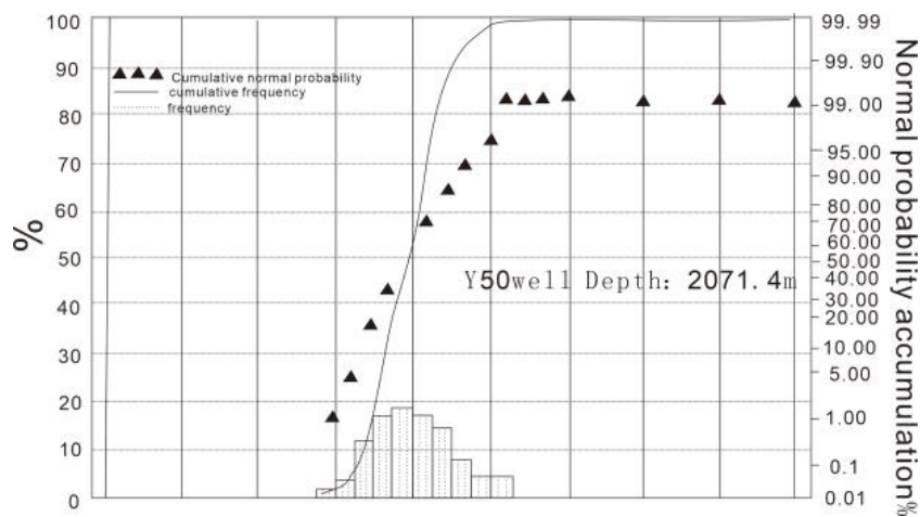
Fig 4. Statistical Chart of Grain Size Distribution of Chang-3 Oil Formation in Baibao Area
