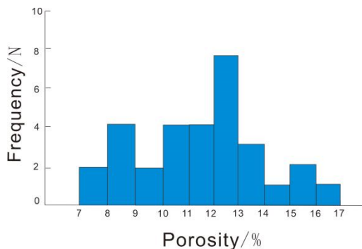
Fig 2. Histogram of Reservoir Porosity Distribution
